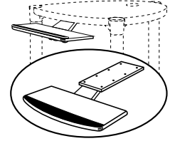
EX 33KB Mechanism Keyboard Tray 745W. x 300D. x 35H. mm. 29 3 / 16 "W. x 12"D. x 1 3 / 8 "H. inch.
