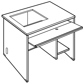
SR 688 (Semi Recess) Computer Workstation 909 x 800 x 750 mm 35 3 / 4 " x 31 1 / 2 " x 29 1 / 2 " inch
