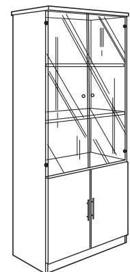
663 CB High Cabinet 810W. x 456D. x 2070H. mm 32"W. x 18"D. x 81 1/2"H. inch
